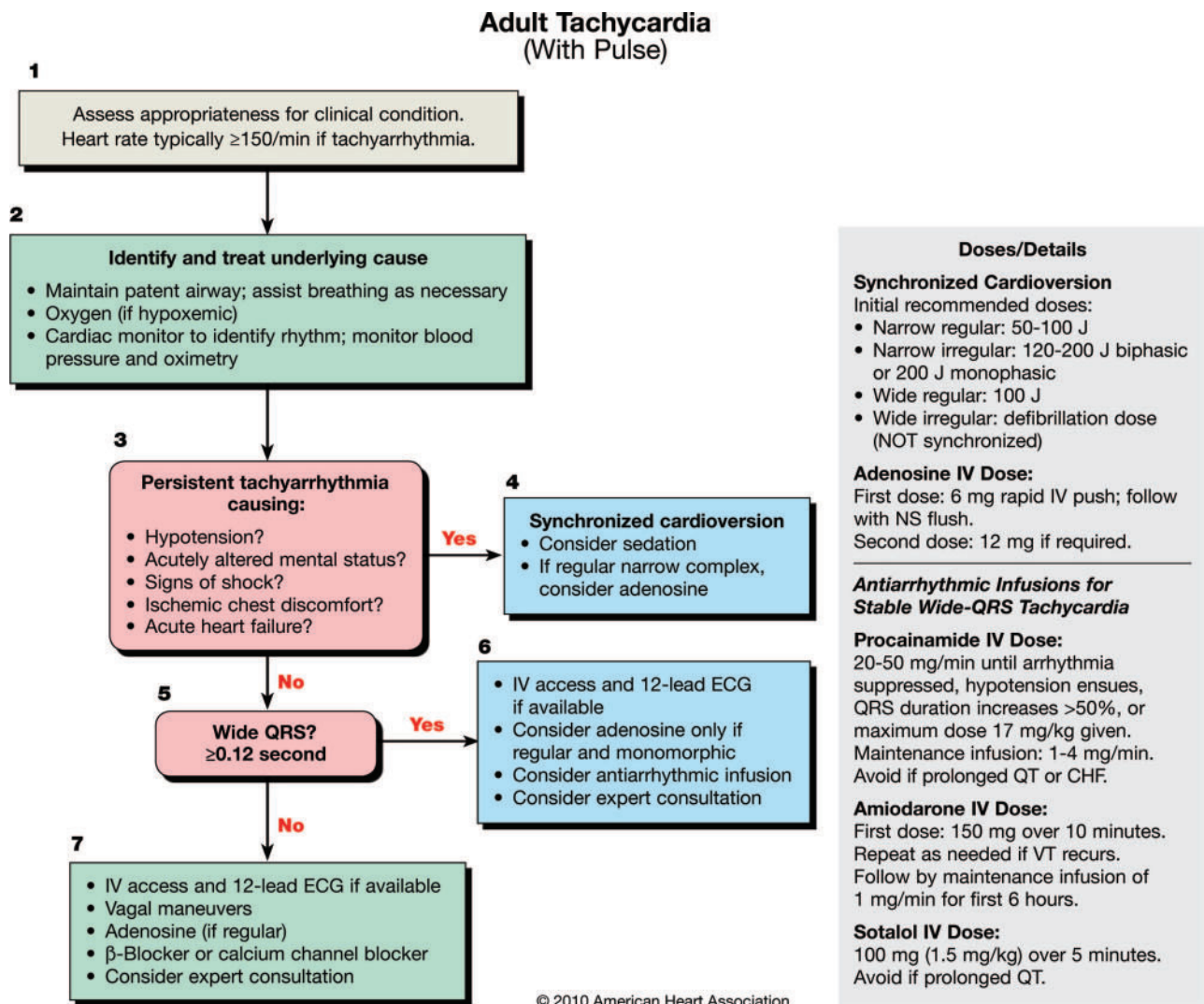
Figure 4. Tachycardia Algorithm.
